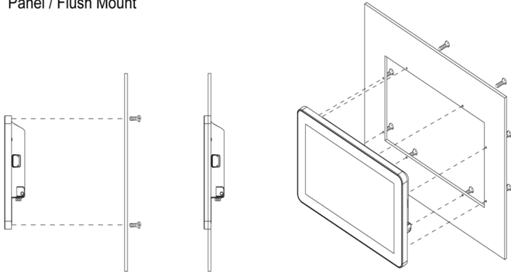
Panel / Flush Mount
